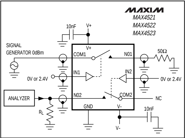
Figure 5. Crosstalk
