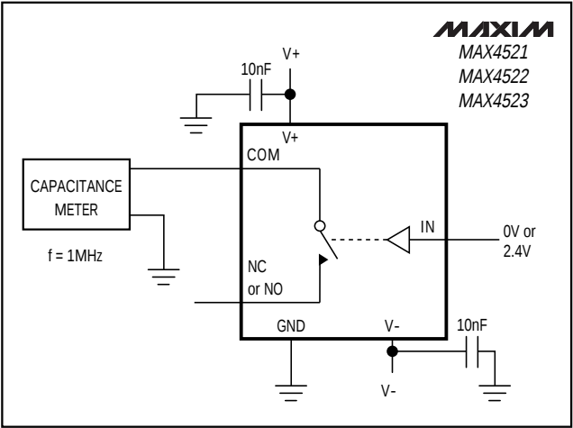
Figure 7. Channel-On Capacitance
