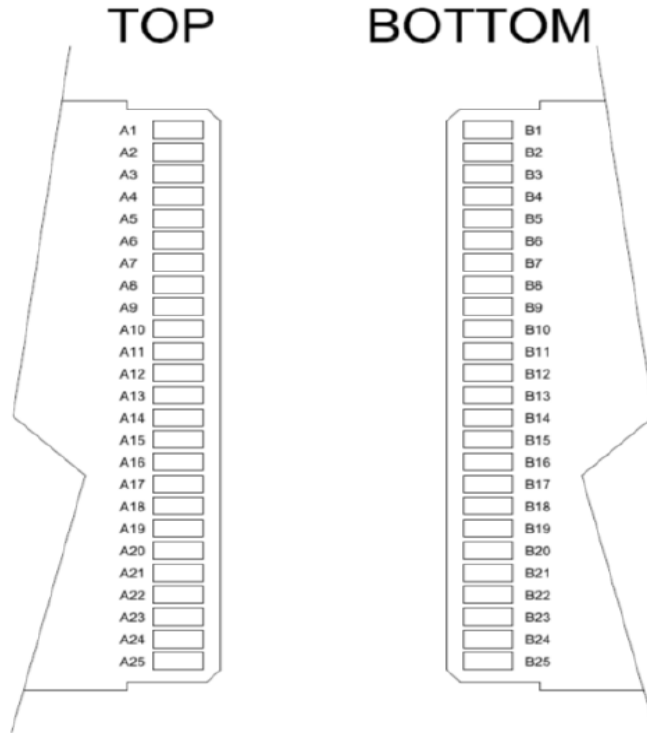
Figure 22. Pin Assignment of DC Output Connector (PCB card edge)
