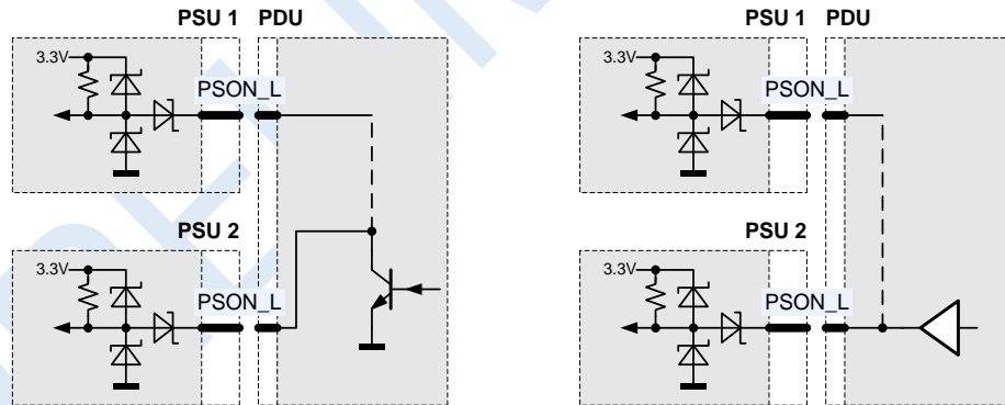
Figure 11. PS_ON Connection
