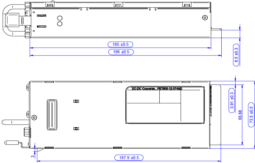
Figure 19. Top and side view with the connector added (TBD)
