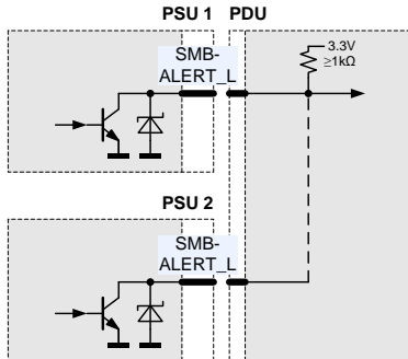
Figure 13. SMBALERT_L connection
