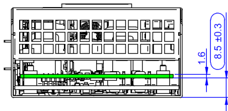
Figure 20. Front View
