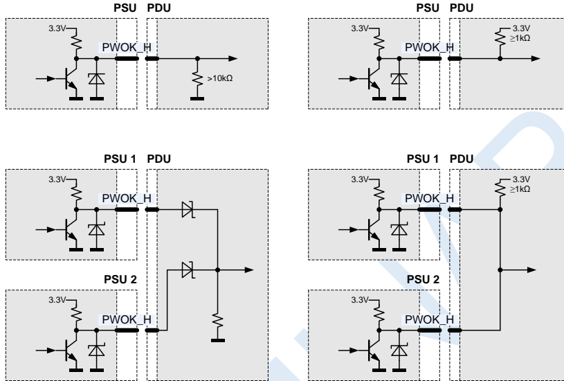
Figure 12. PWOK Connection
