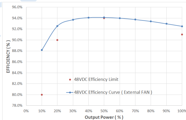
Figure 2. Efficiency Curve (To be updated)
