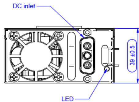
Figure 21. Rear View
