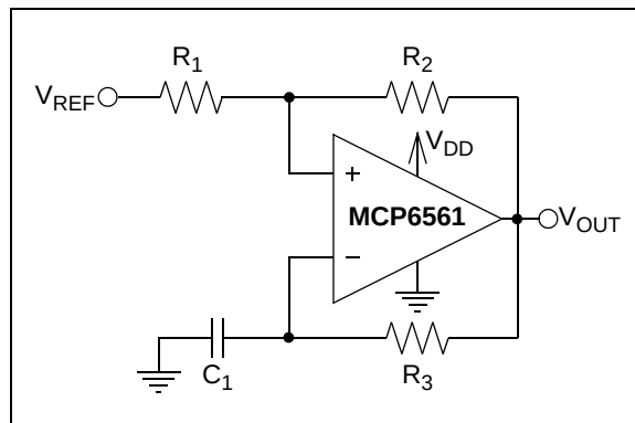
FIGURE 4-14: Bistable Multi-vibrator.
