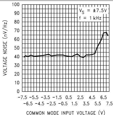
Figure 23. Input Voltage Noise vs Input Voltage
