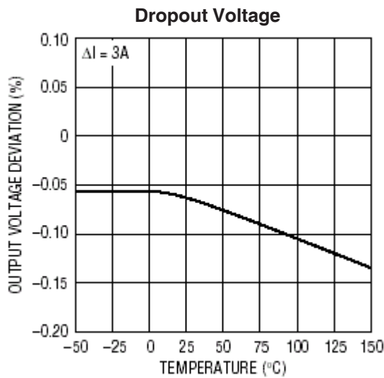
Fig 3: Typical Output Voltage Deviation Vs Temperature
