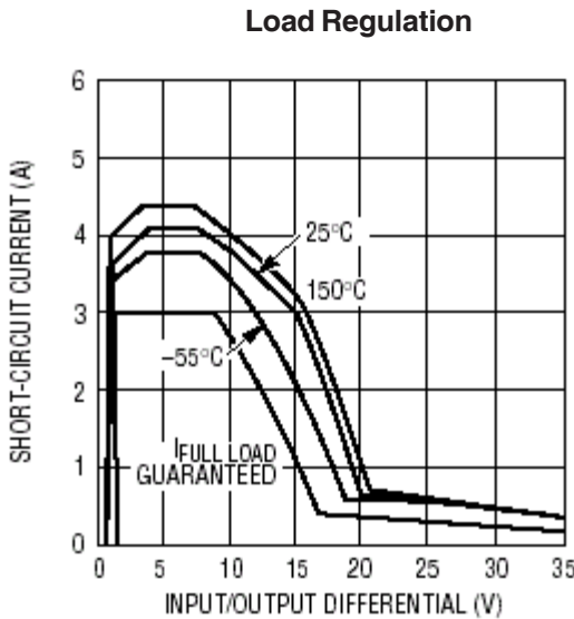
Fig 2: Typical Short Circuit Current Vs Input/Output Differential
