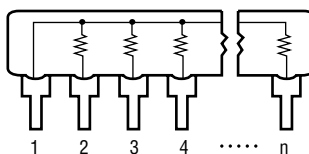
-1 Circuit Bussed Resistors
