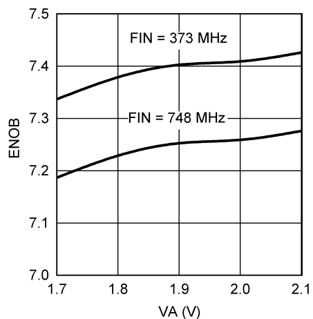
ENOB vs. SUPPLY VOLTAGE
