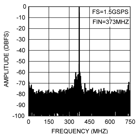
Spectral Response at FIN = 373 MHz
