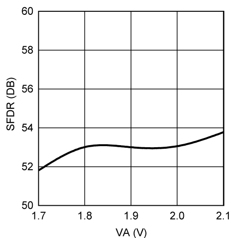
SFDR vs. SUPPLY VOLTAGE
