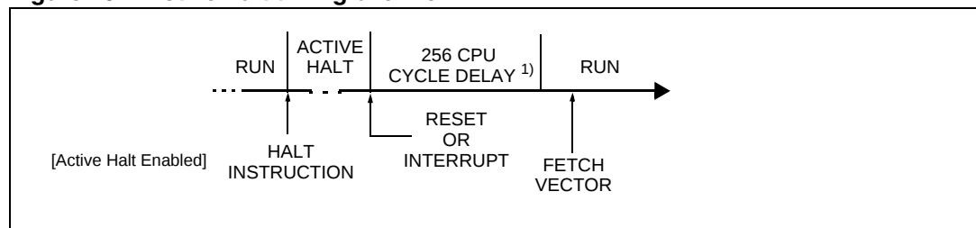
Figure 20. Active-halt timing overview
