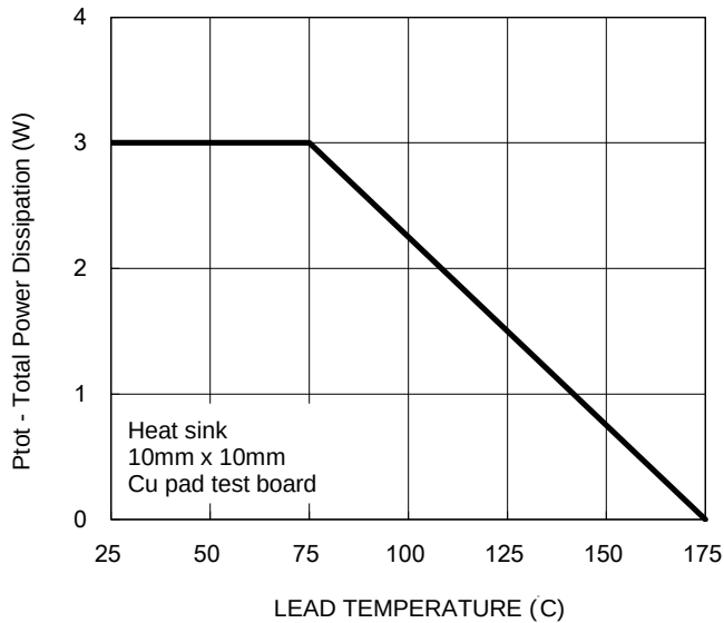
Fig.1 Steady State Power Durling
