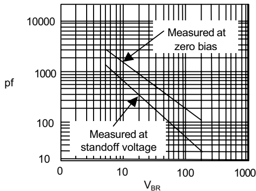
Figure 3 - Typical Capacitance
