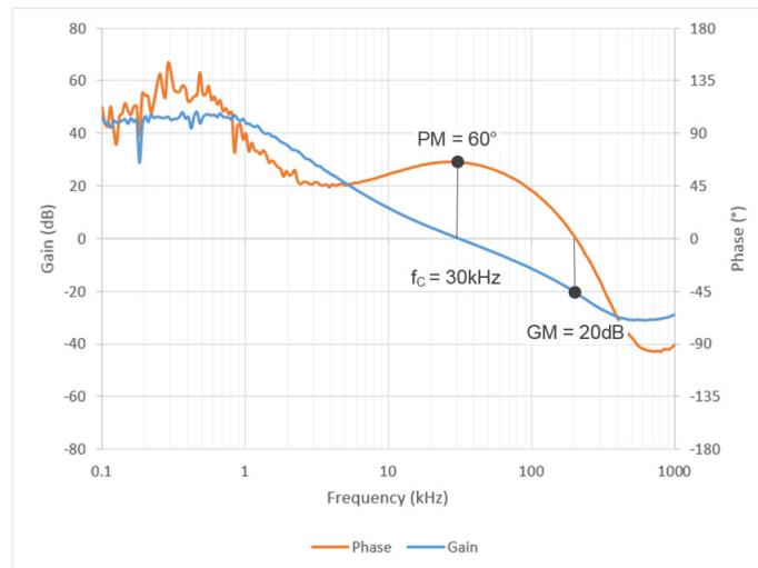
Figure 13: Bode plot measurement of the complete system R_Z = 8.25 \text{ k}\Omega , C_Z = 2.2 \text{ nF} , C_P = 100 \text{ pF} , L_1 = 10 \text{ }\mu\text{H} , C_{OUT} = 2 \times 10 \text{ }\mu\text{F} Ceramic
