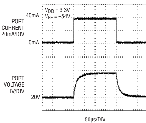
Classification Transient Response to 40mA Load Step
