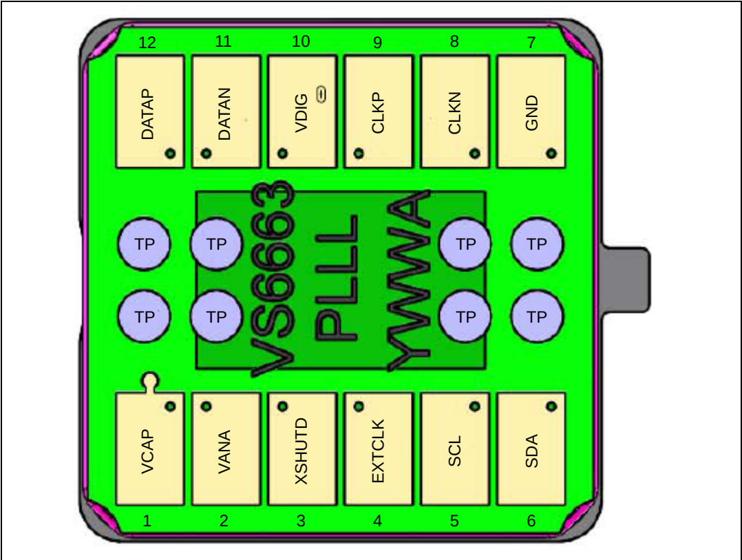
Figure 4. VS6663 module pinout (viewed from bottom of camera module)
