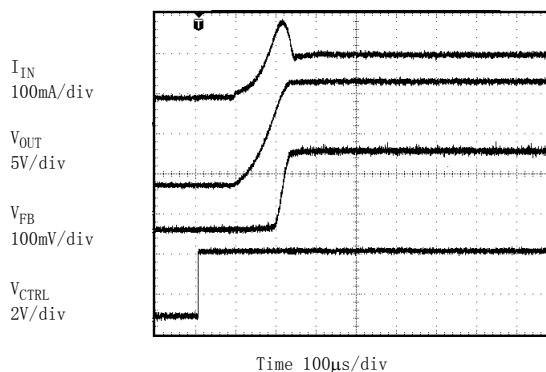
Figure 19. Soft Start Waveform V IN =3.6V, 5 LEDs, I LED =20mA
