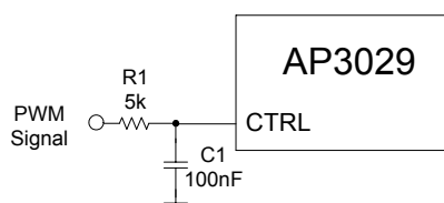
Figure 22. Dimming Control Using a Filtered PWM Signal Voltage in CTRL Pin
