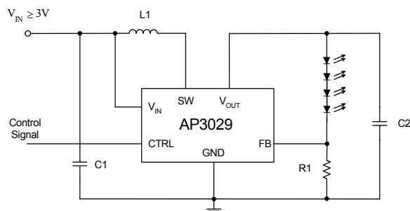
Figure 18. Typical Application circuit to Decide R1
