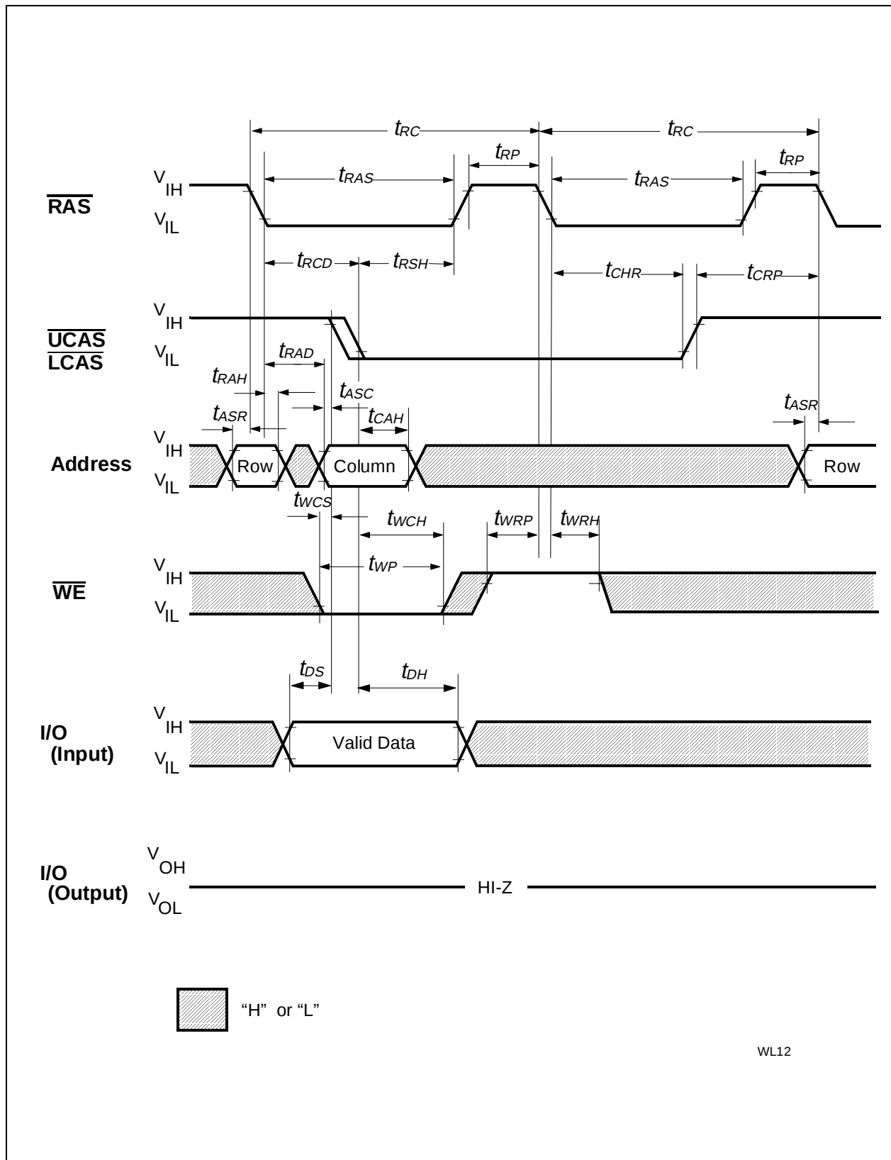
Hidden Refresh Write Cycle
