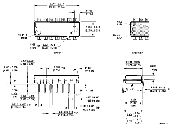
Order Number MM74HC74N NS Package N14A
