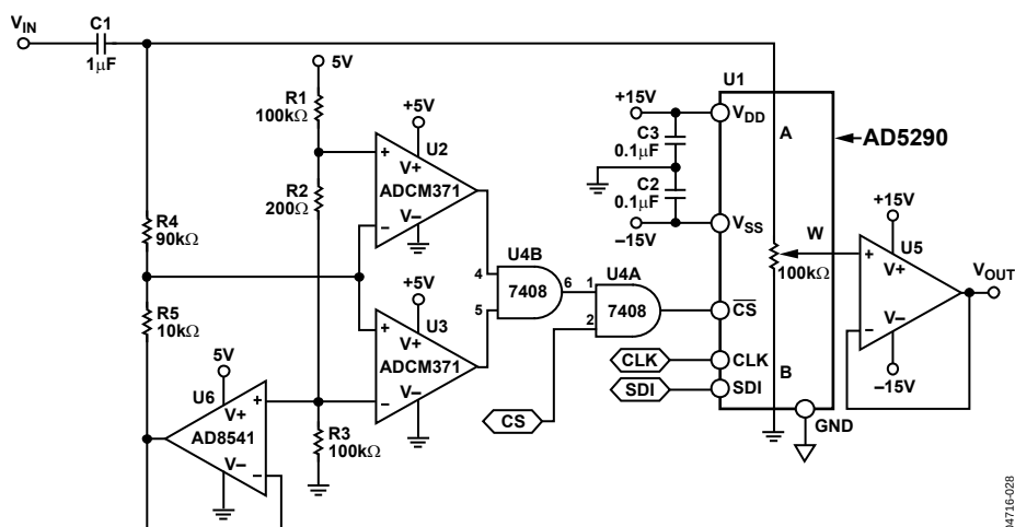
Figure 35. Audio Volume Control with Zipper Noise Reduction
