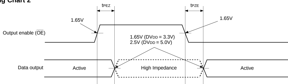
Timing Chart 2
