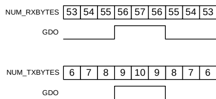
Figure 19: FIFO_THR=13 vs. Number of Bytes in FIFO ( GD0x_CFG=0x00 in RX and GD0x_CFG=0x02 in TX)
