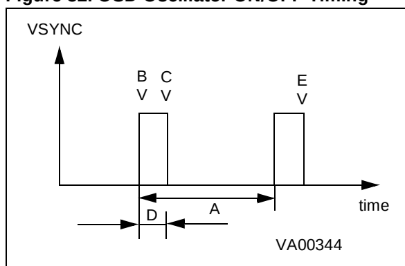
Figure 32. OSD Oscillator ON/OFF Timing
