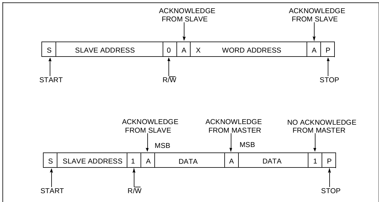
Figure 25. I 2 C Master Reads After Setting Slave Register Address (Write Address, Read Data)
