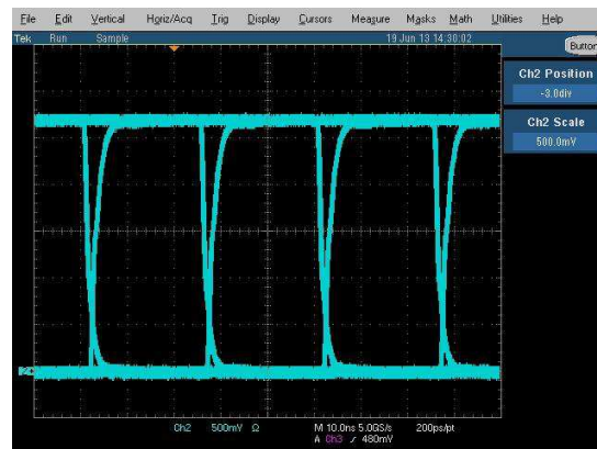
Figure 17. Eye Diagram at 40 Mbps, 2.7V at 25^\circ\text{C}
