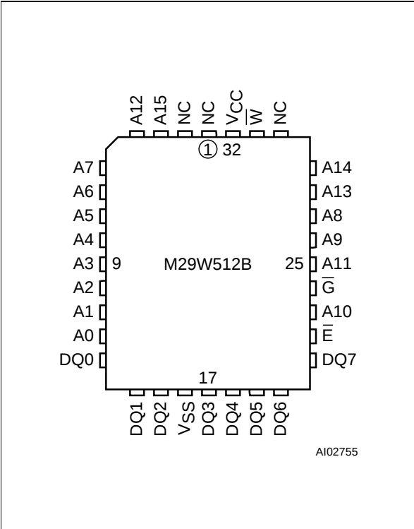
Figure 3. PLCC Connections
