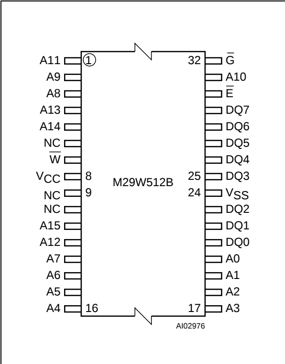
Figure 2. TSOP Connections
