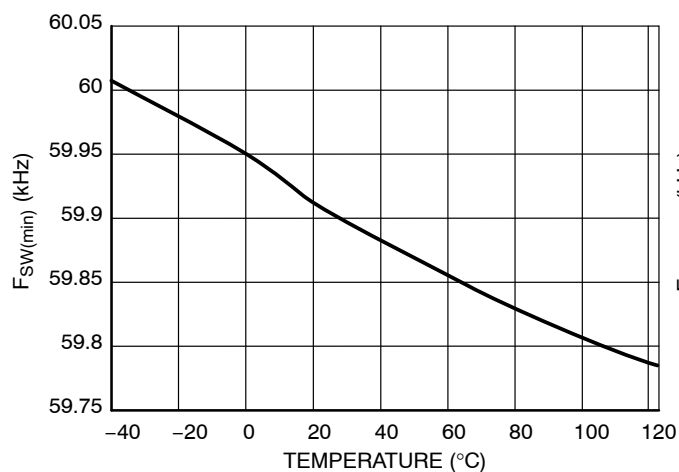
Figure 6. F SW(min) Frequency Clamp
