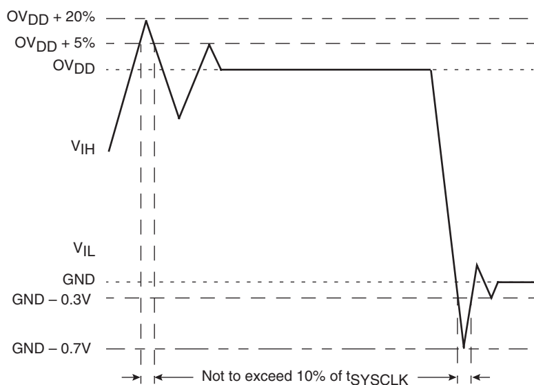
Figure 6-1. Overshoot/Undershoot Voltage
