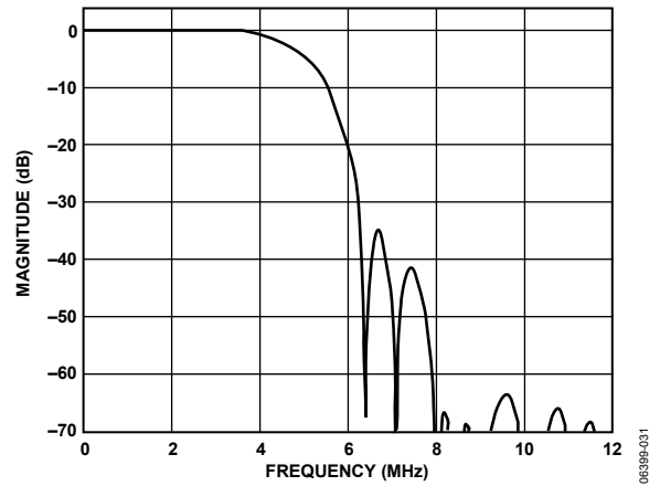
Figure 31. SD PAL, Luma Low-Pass Filter Response
