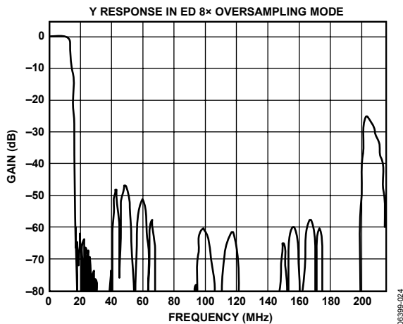
Figure 24. ED 8× Oversampling, Y Filter Response
