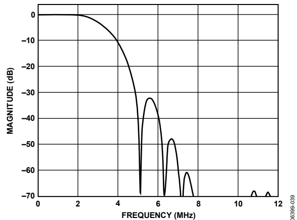
Figure 39. SD Luma CIF Low-Pass Filter Response
