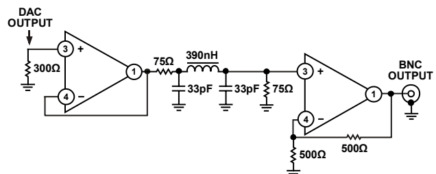
Figure 86. Example of Output Filter for HD, 4 \times Oversampling
