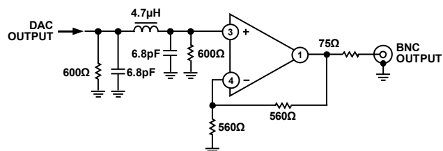
Figure 85. Example of Output Filter for ED, 8 \times Oversampling
