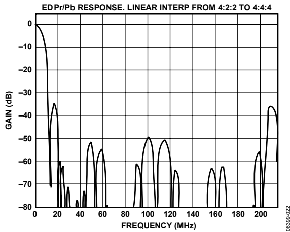
Figure 22. ED 8× Oversampling, PrPb Filter (Linear) Response
