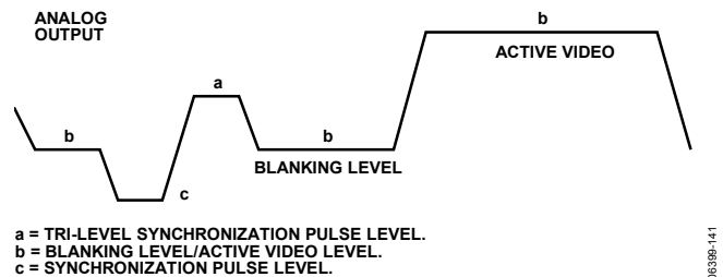
Figure 59. ED/HD Nonstandard Timing Mode Output Levels
