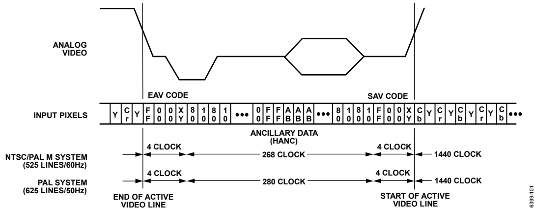
Figure 100. SD Slave Mode 0
