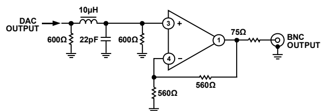
Figure 84. Example of Output Filter for SD, 16 \times Oversampling
