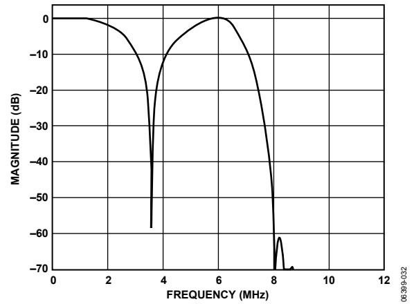
Figure 32. SD NTSC, Luma Notch Filter Response
