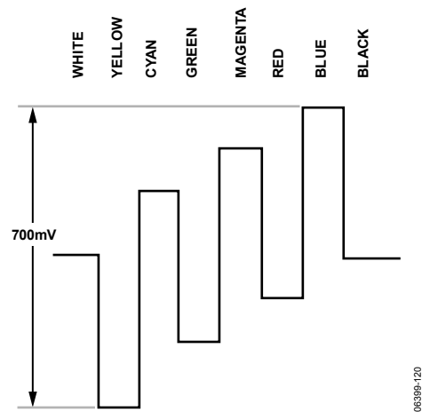
Figure 119. Pb Levels—PAL
