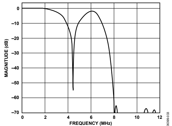
Figure 33. SD PAL, Luma Notch Filter Response
