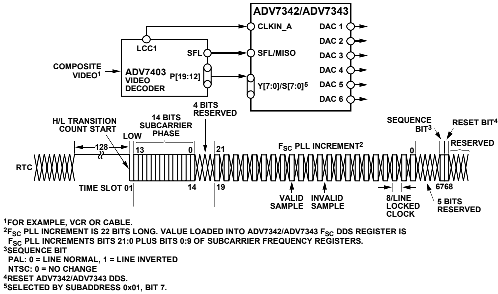
Figure 62. SD Subcarrier Frequency Lock Timing and Connections Diagram (Subaddress 0x84, Bits [2:1] = 11)
