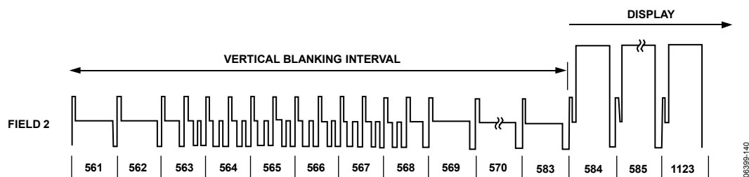
Figure 139. SMPTE 274M (1080i)
