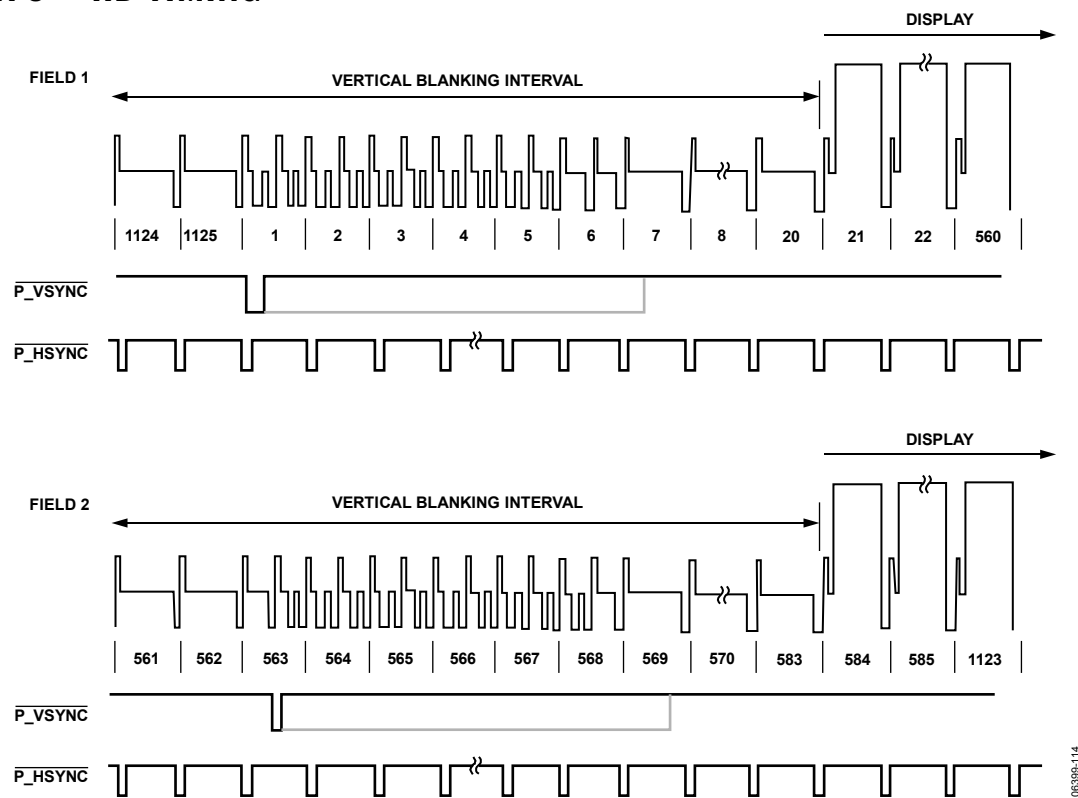
Figure 113. 1080i HSYNC and VSYNC Input Timing
