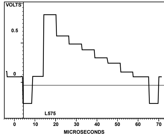
Figure 132. PAL Luma
