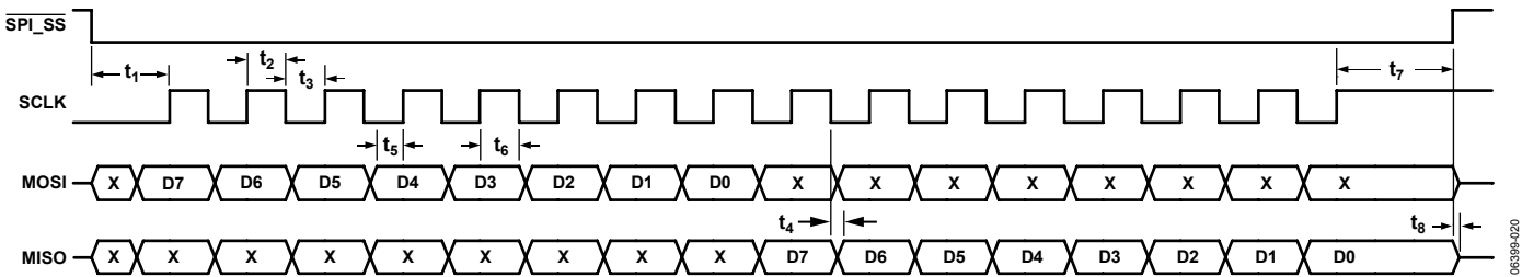
Figure 20. MPU Port Timing Diagram (SPI Mode)
