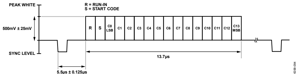
Figure 93. Enhanced Definition (625p) CGMS Waveform
