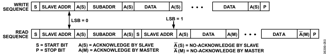
Figure 50. I²C Read and Write Sequence
