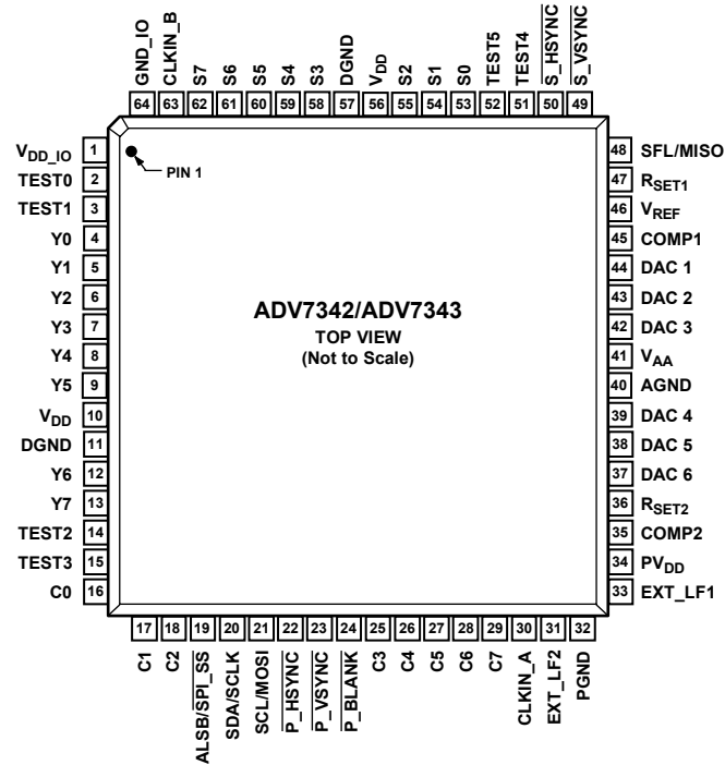
Figure 21. Pin Configuration
