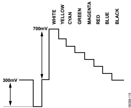
Figure 114. Y Levels—NTSC
