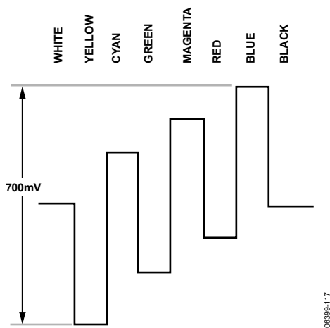
Figure 116. Pb Levels—NTSC
