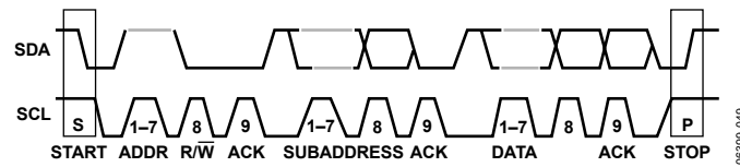
Figure 49. I²C Data Transfer
