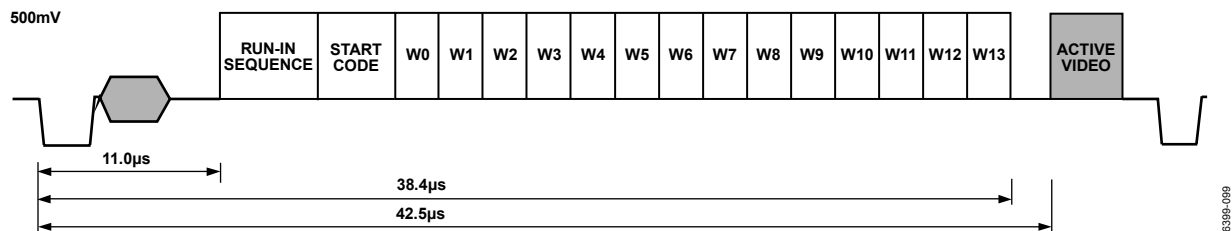
Figure 98. WSS Waveform Diagram
