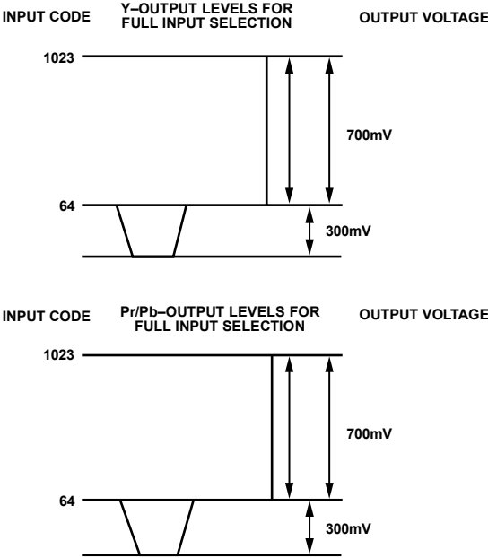
Figure 123. Output Levels for Full Input Selection
