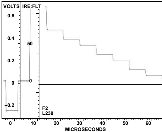
Figure 129. NTSC Luma
