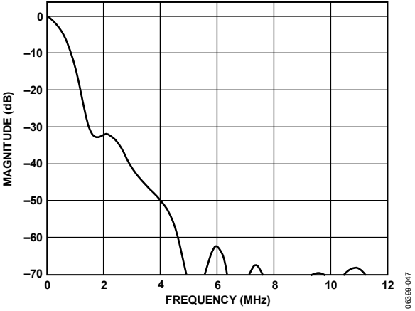
Figure 47. SD Chroma QCIF Low-Pass Filter Response
