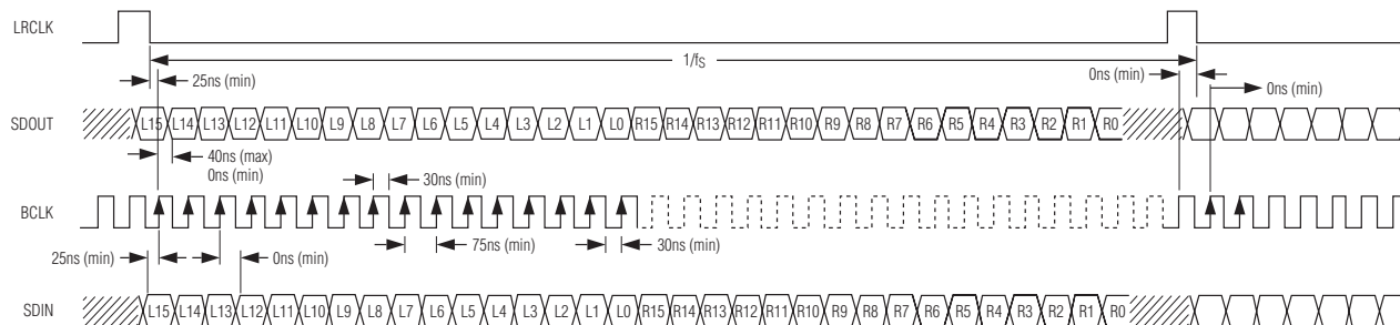
Figure 4. Digital Audio Interface Voice Slave Mode Examples
