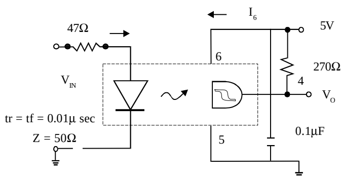
SWITCHING TEST CIRCUIT
