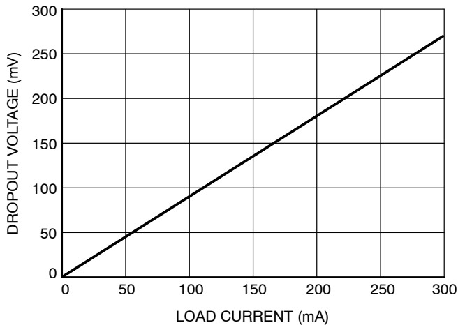
Figure 13. Dropout vs. Load Current
