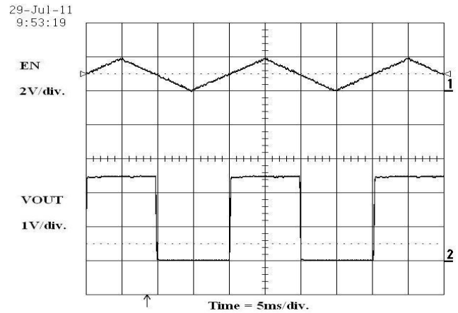
Figure 22. Slow-Enable Operation (300 mA Load)
