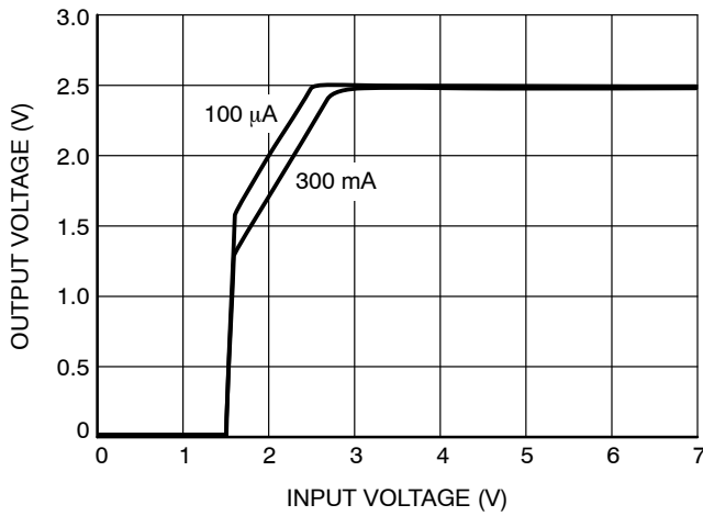
Figure 3. Dropout Characteristics
