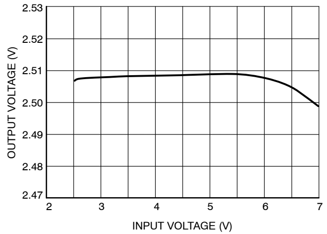
Figure 4. Line Regulation
