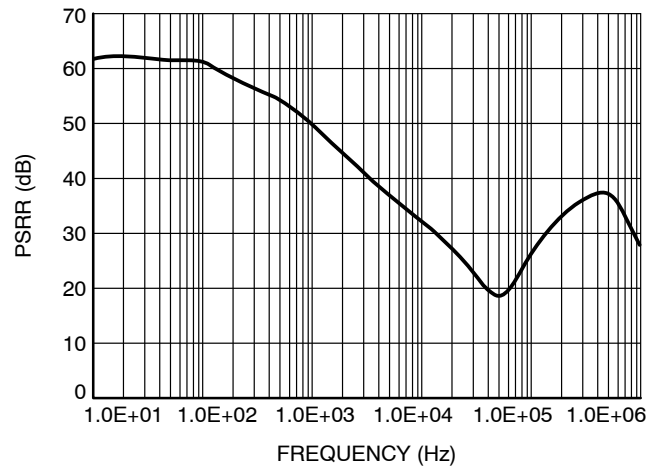
Figure 10. PSRR vs. Frequency (10 mA Load)
