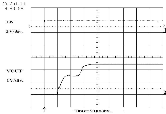
Figure 17. Enable Turn-On (300 mA Load)
