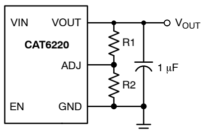
Figure 2. R1 and R2 Set CAT6220's Output Voltage
