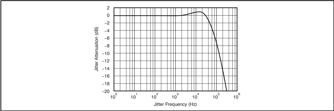
Figure 69. DIR Jitter Attenuation Characteristics
