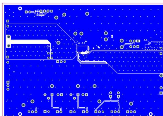
图 64. bq25871 Layout Diagram (Bottom 1)
