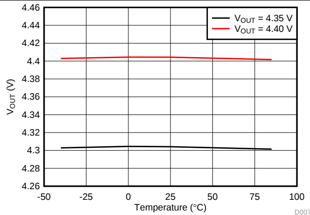
图 7. VOUT Regulation vs Temperature
