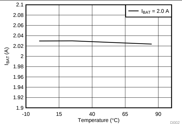
图 2. IBAT ADC vs Temperature at 2 A
