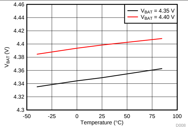
图 8. VBAT Regulation vs Temperature
