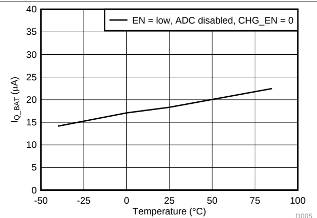
图 5. Quiescent Current with Battery Only vs Temperature
