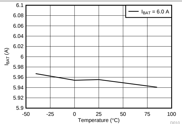
图 10. IBAT Regulation vs Temperature at 6 A
