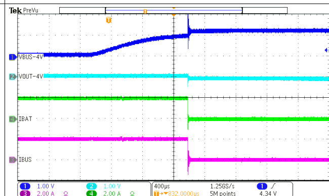
图 58. IBUS OCP During Load Transient
