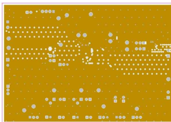
图 63. bq25871 Layout Diagram (Mid Layer 1)
