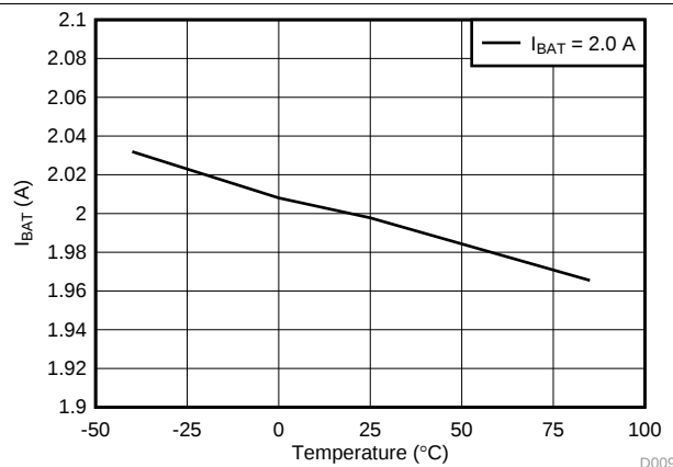
图 9. IBAT Regulation vs Temperature at 2 A
