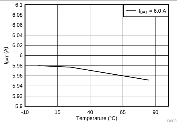
图 3. IBAT ADC vs Temperature at 6 A
