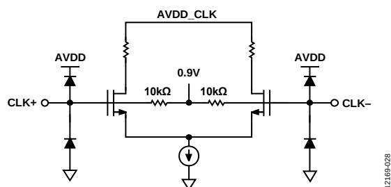
Figure 43. Equivalent Clock Input Circuit
