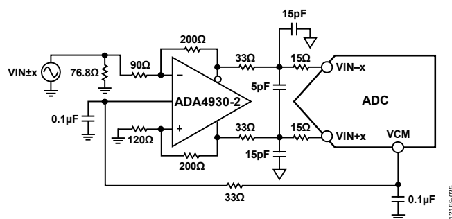
Figure 53. Differential Input Configuration Using the ADA4930-2
