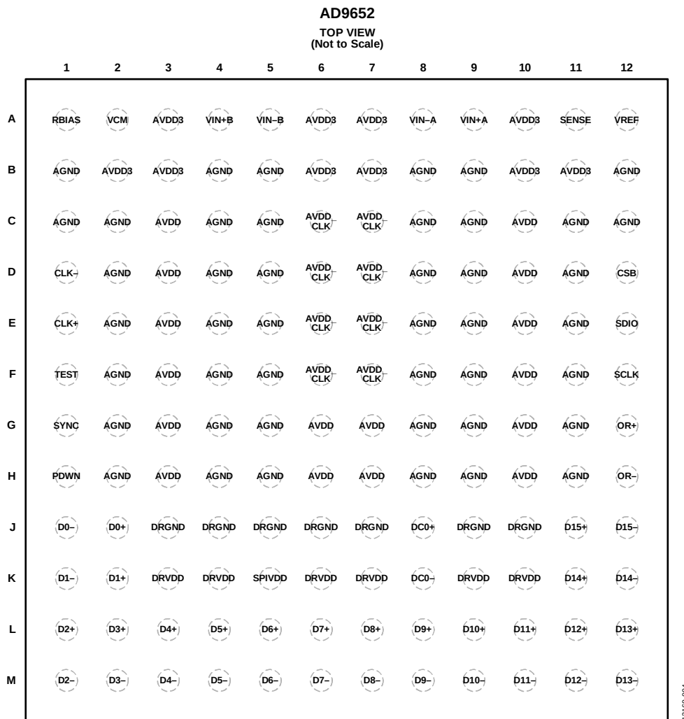
Figure 5. Pin Configuration
