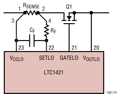
Figure 10. Short-Circuit Protection Circuit
