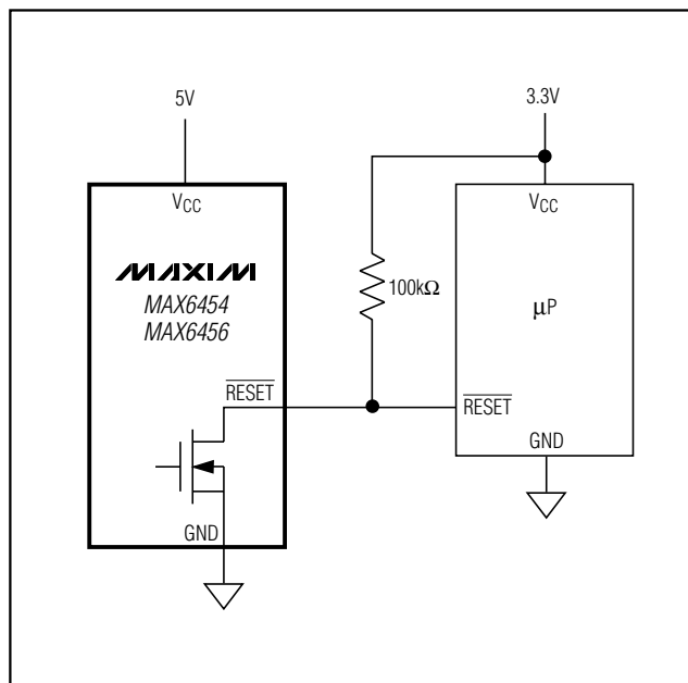
Figure 5. Interfacing to Other Voltage Levels
