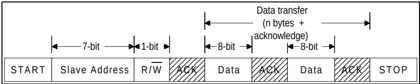
Figure 7-24. Bus Protocol
