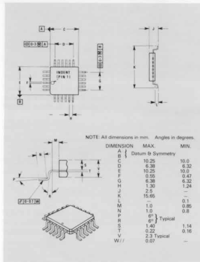
Fig. 10 FX214LG and FX224LG 24-pin Package
