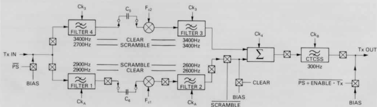
Fig. 5 Basic Tx Path
