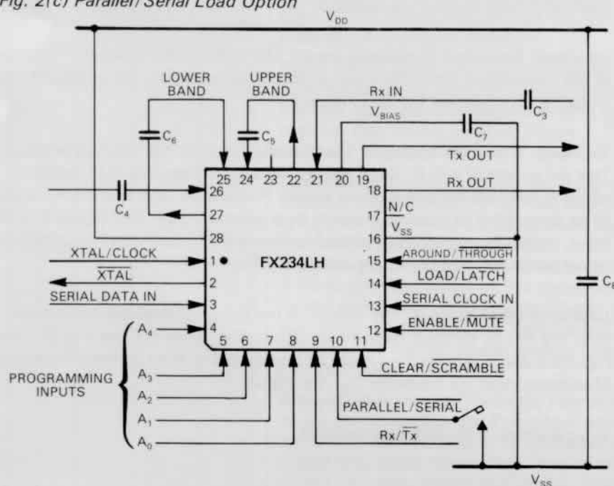
Fig. 2 External Component Connections
