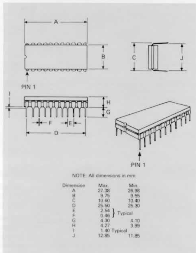
Fig. 8 FX214J 22-pin DIL Package
