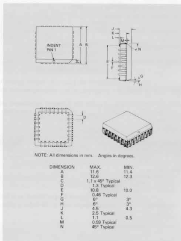
Fig. 11 FX234LH 28-lead Package
