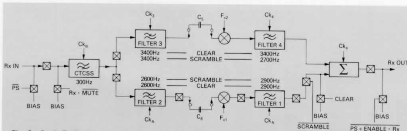
Fig. 6 Basic Rx Path
