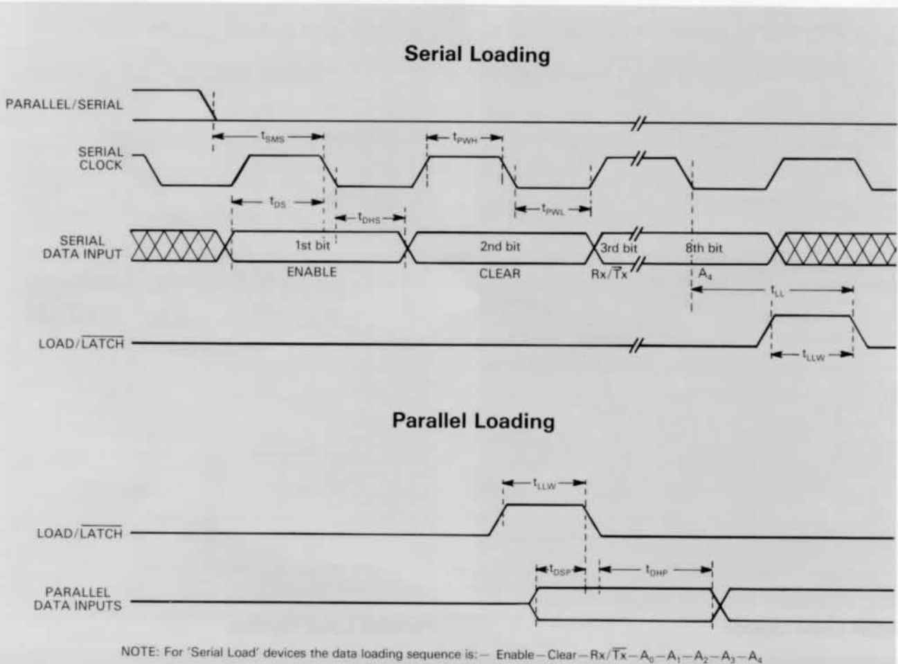
Fig. 7 Loading Timing Diagram
