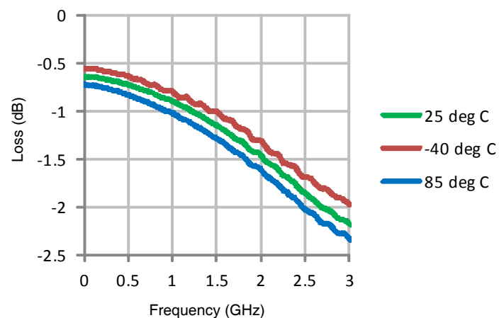
Figure 5. Insertion Loss vs Temperature (RFX-RFC)
