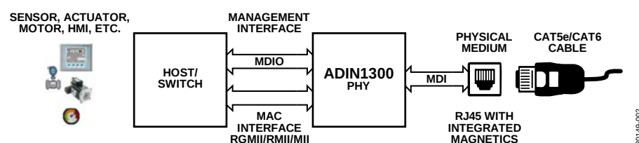
Figure 3. Typical Networked Sensor with PHY Device
