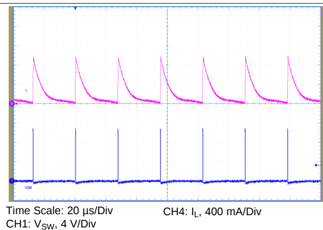
图 36. Short Circuit, PFM, I_{LIM} = 750\text{ mA}
