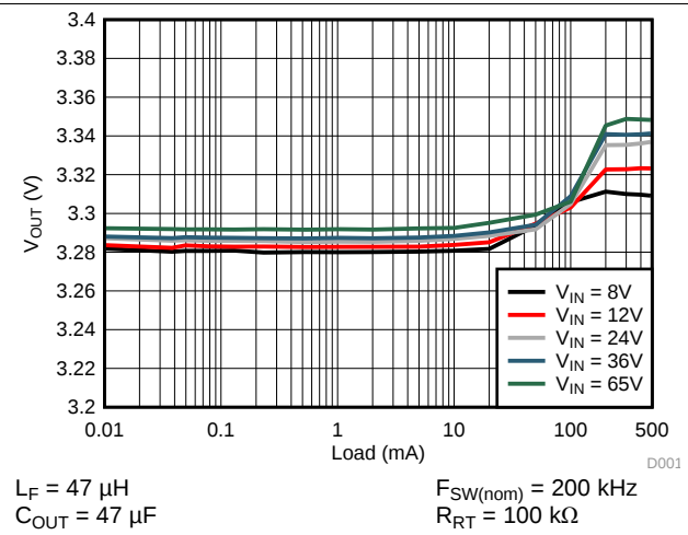
图 65. Converter Regulation
