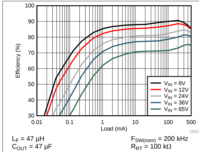
图 64. Converter Efficiency
