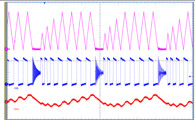
图 38. Full-Load Switching Waveforms PFM Mode, I_{LIM} = 1.25\text{ A} , Modulated
