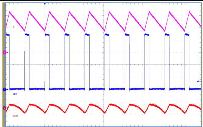
Time Scale: 10 μs/Div CH1: V_{SW} , 5 V/Div CH2: V_{OUT} , 50 mV/Div CH4: I_L , 200 mA/Div
