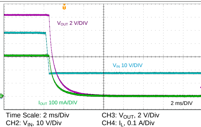
图 88. Shutdown Waveforms
