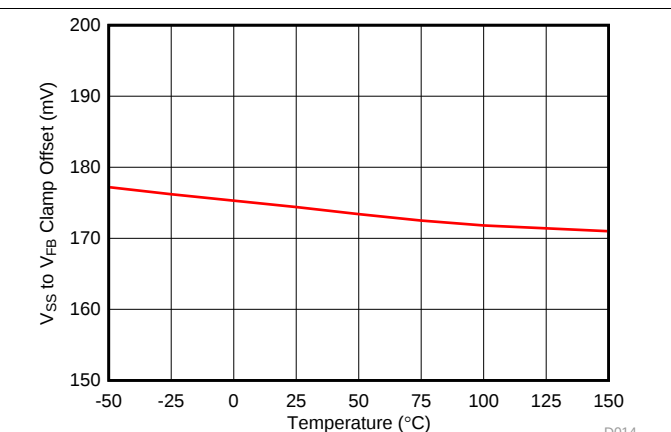
图 49. Soft-Start to Feedback Clamp Offset vs Temperature
