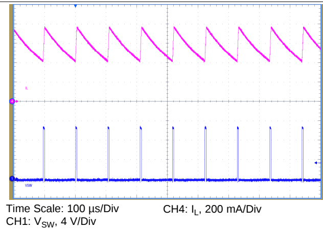
图 32. Short Circuit, COT, Type 2
