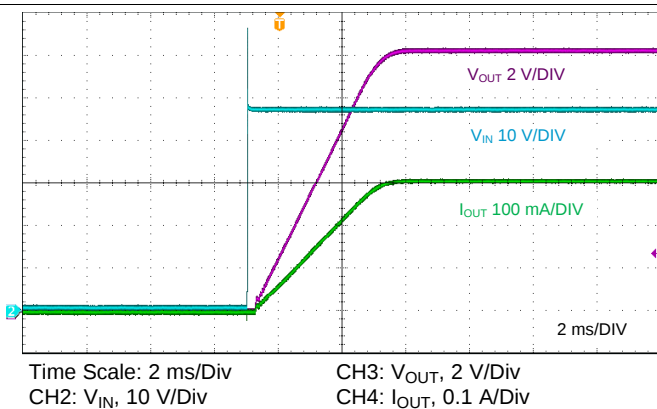
图 87. Start-up Waveforms
