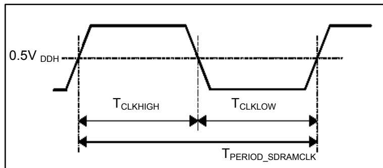
Figure 5. SDR DRAM Clock Specifications-1
