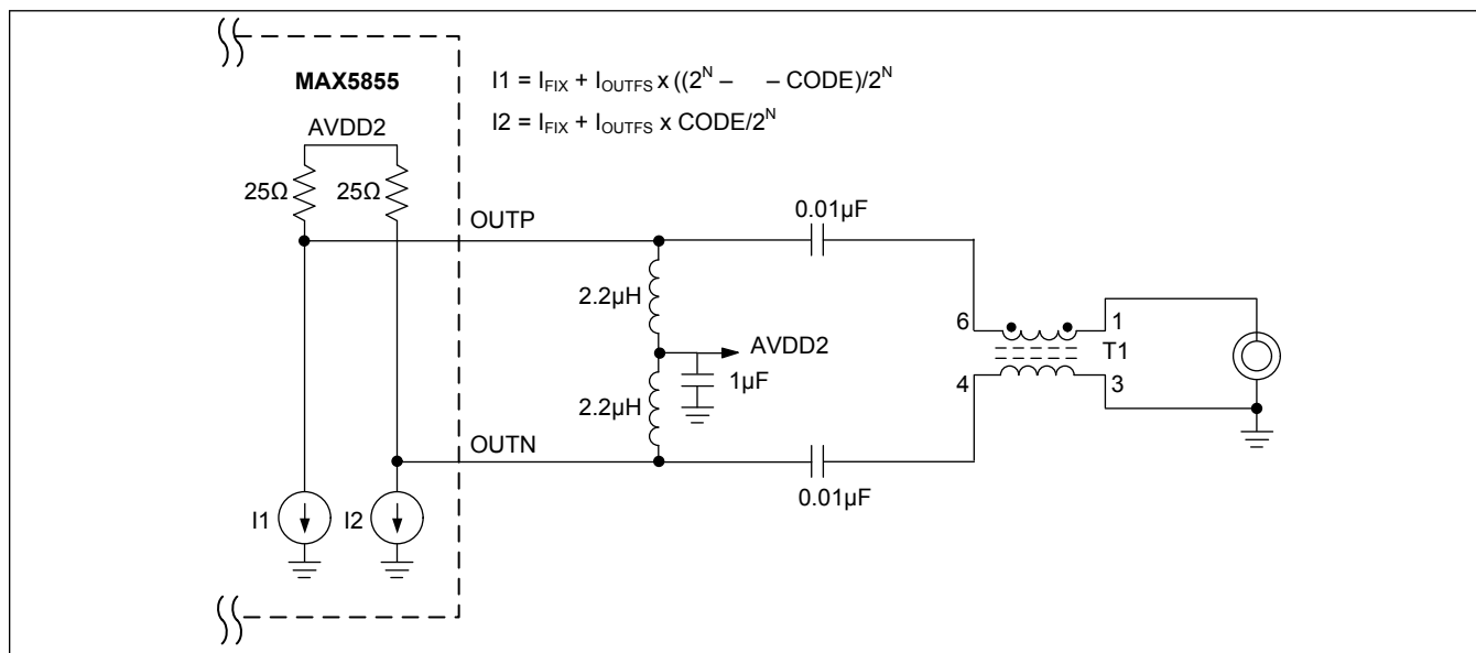
Figure 25. Typical DAC Output Configuration
