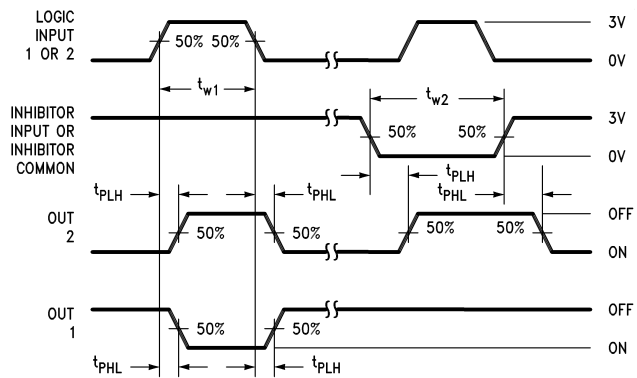
FIGURE 2. AC Waveforms
