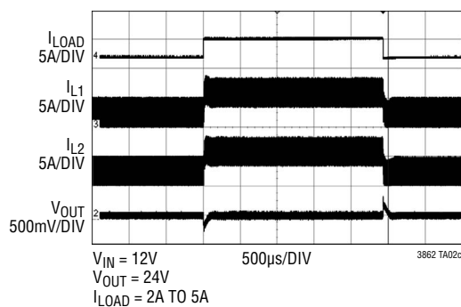
Load Step
