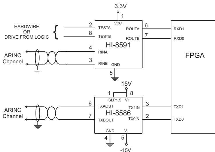
FIGURE 2 - APPLICATION DIAGRAM
