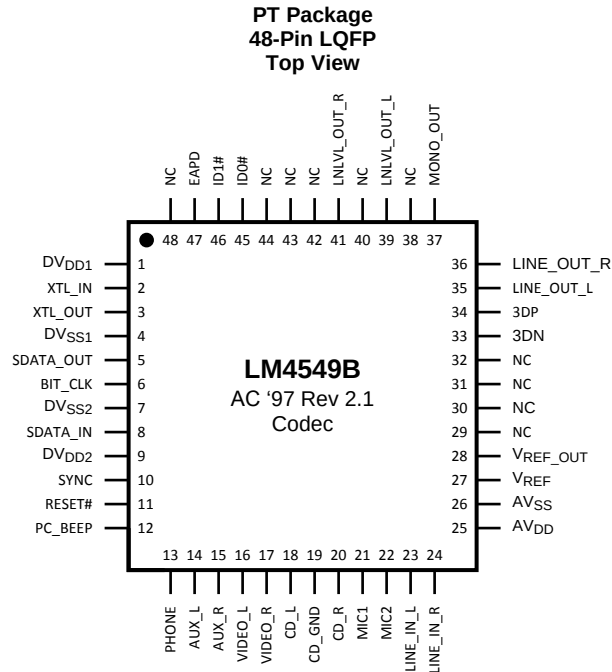
Pin Functions
