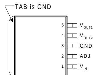
DF PACKAGE (Top View)
