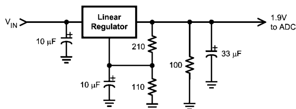
FIGURE 18. Non-Spiking Power Supply
