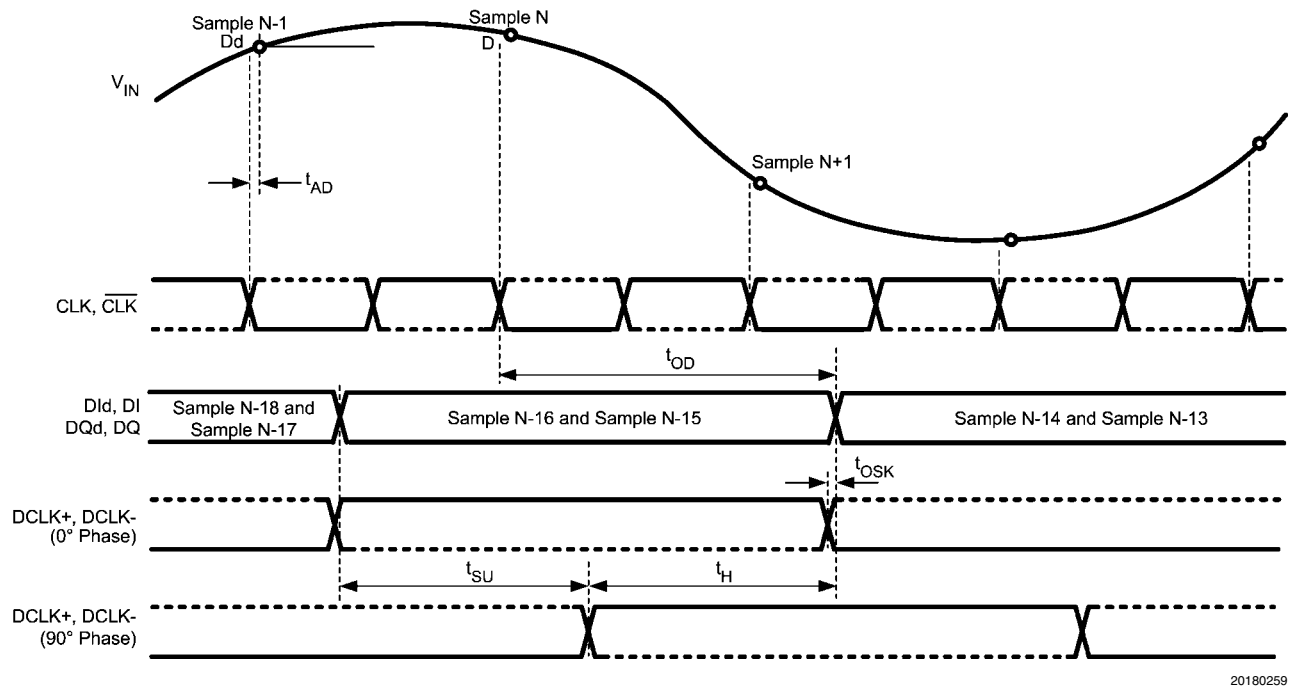
FIGURE 4. ADC08D1000 Timing — DDR Clocking
