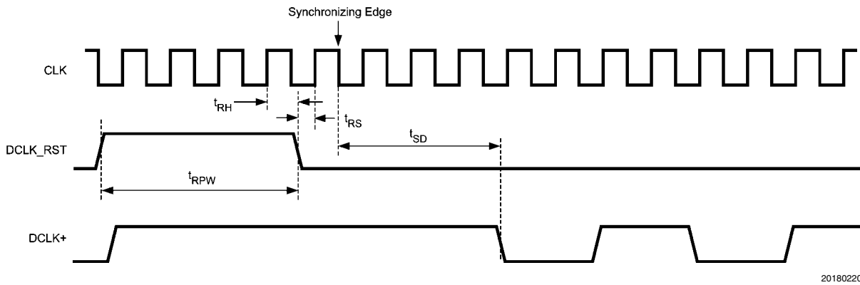
FIGURE 6. Clock Reset Timing in DDR Mode
