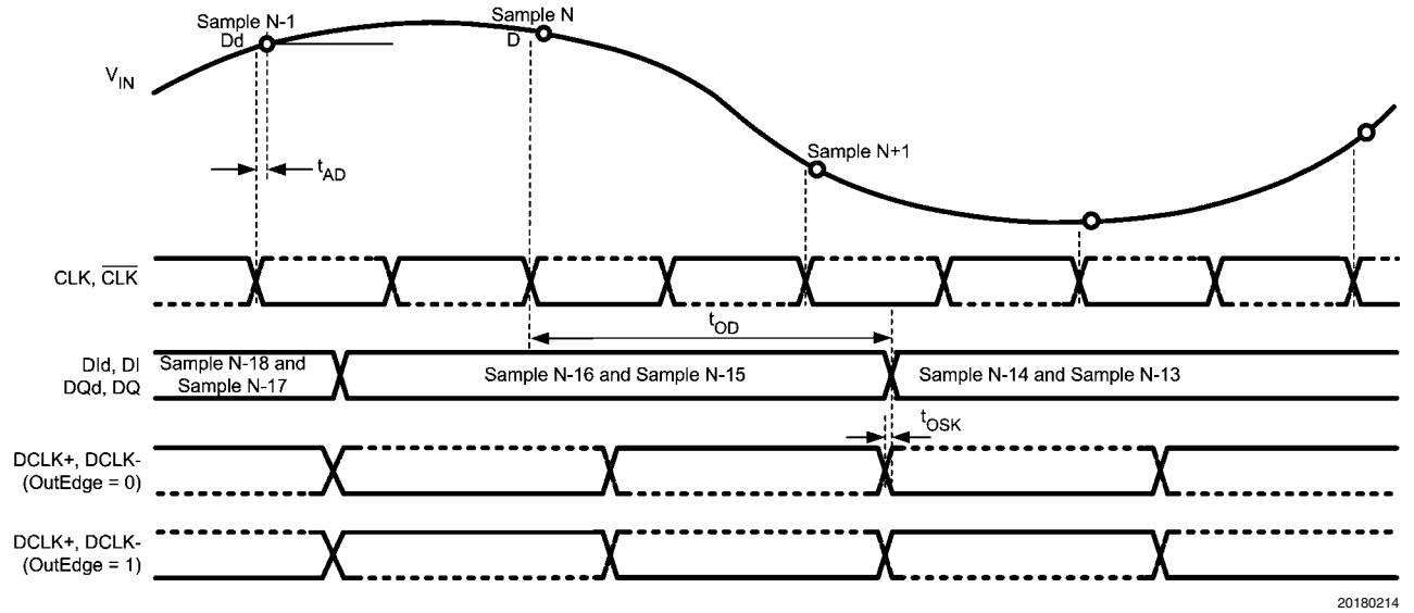
FIGURE 3. ADC08D1000 Timing — SDR Clocking
