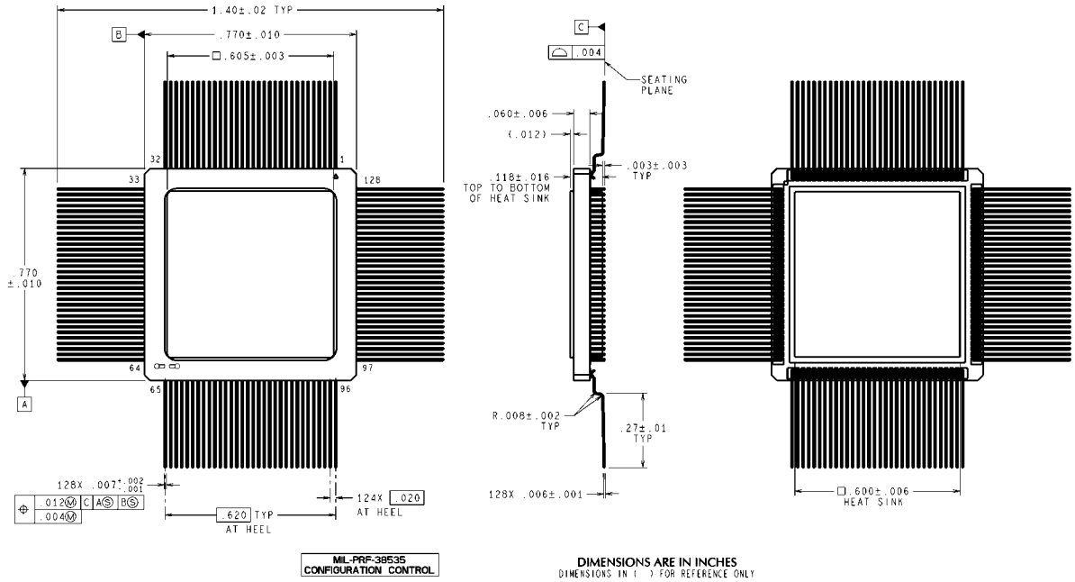
128-Lead Ceramic Quad (Gold Lead Finish) NS Package Number EL128A
