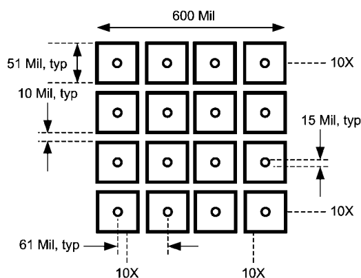
FIGURE 19. Recommended Package Land Pattern
