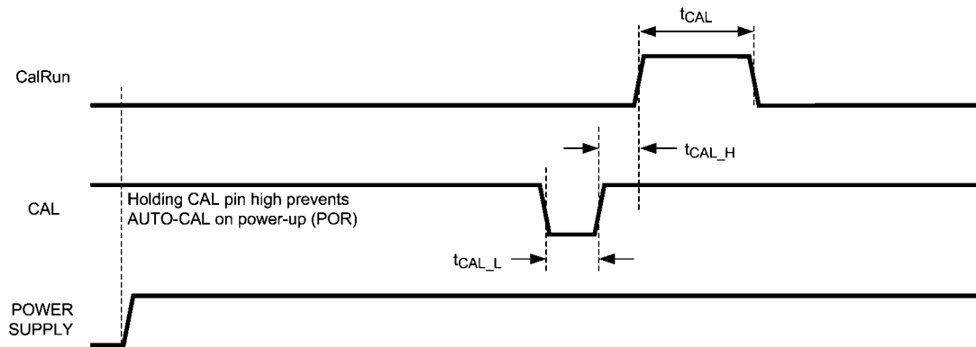
FIGURE 10. For On-Command Calibration Only (See para. 2.1, The Cal Pin)
