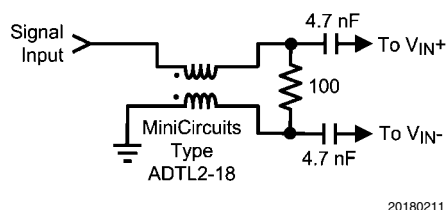
FIGURE 14. Single-Ended To Differential Signal Conversion With A Balun-Connected Transformer
