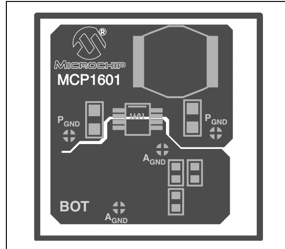
FIGURE 5-4: Bottom Layer.
