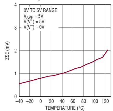
Single-Supply Zero-Scale Error vs Temperature
