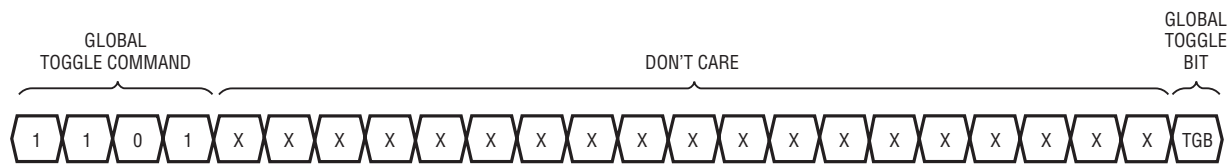
Figure 7. Global Toggle Syntax
