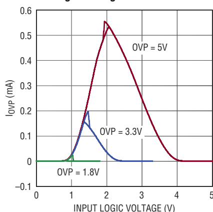
IOVP Supply Current vs Logic Voltage
