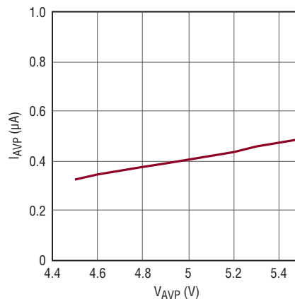
AVP Shutdown Current vs AVP
