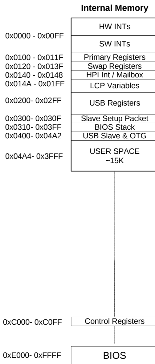
Figure 6. Memory Map
