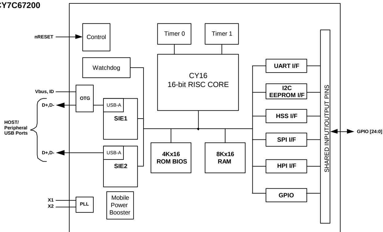
Block Diagram CY7C67200
