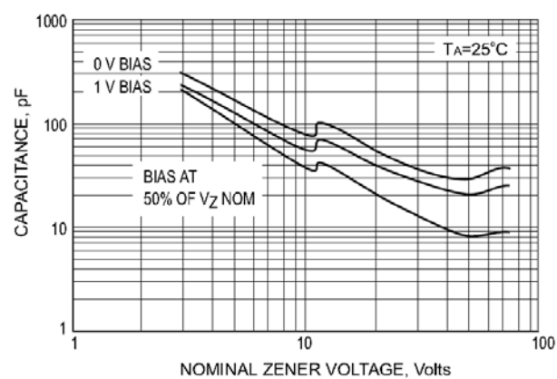
Fig.4 TYPICAL CAPACITANCE
